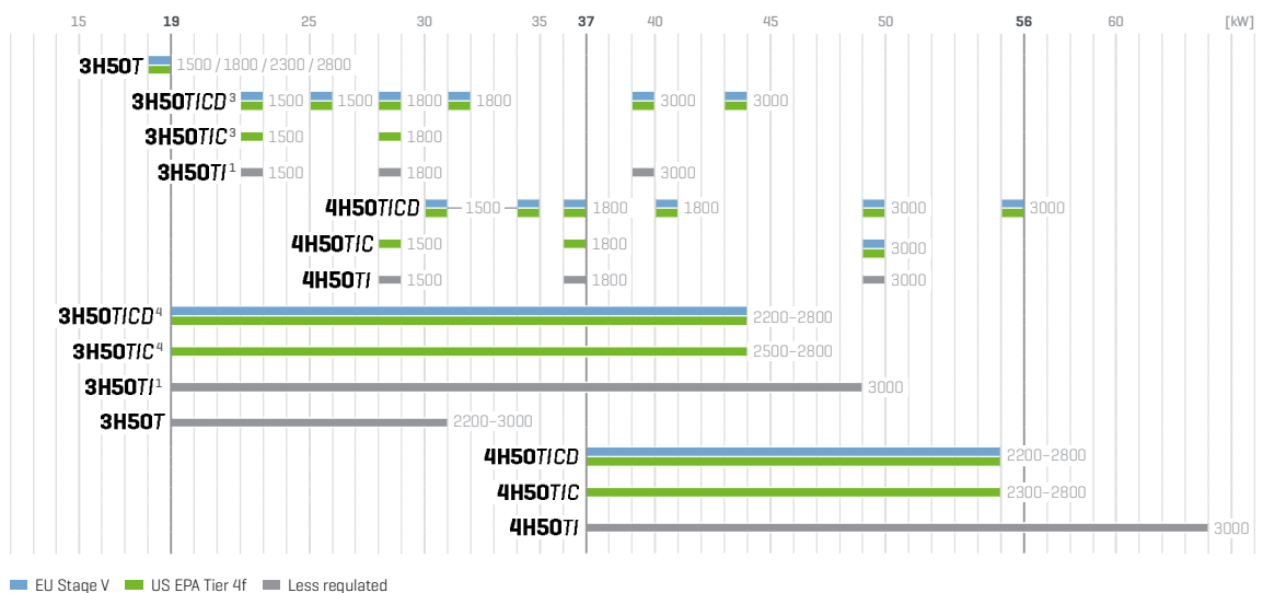
H-series – power ranges, emission classes and rated speeds
